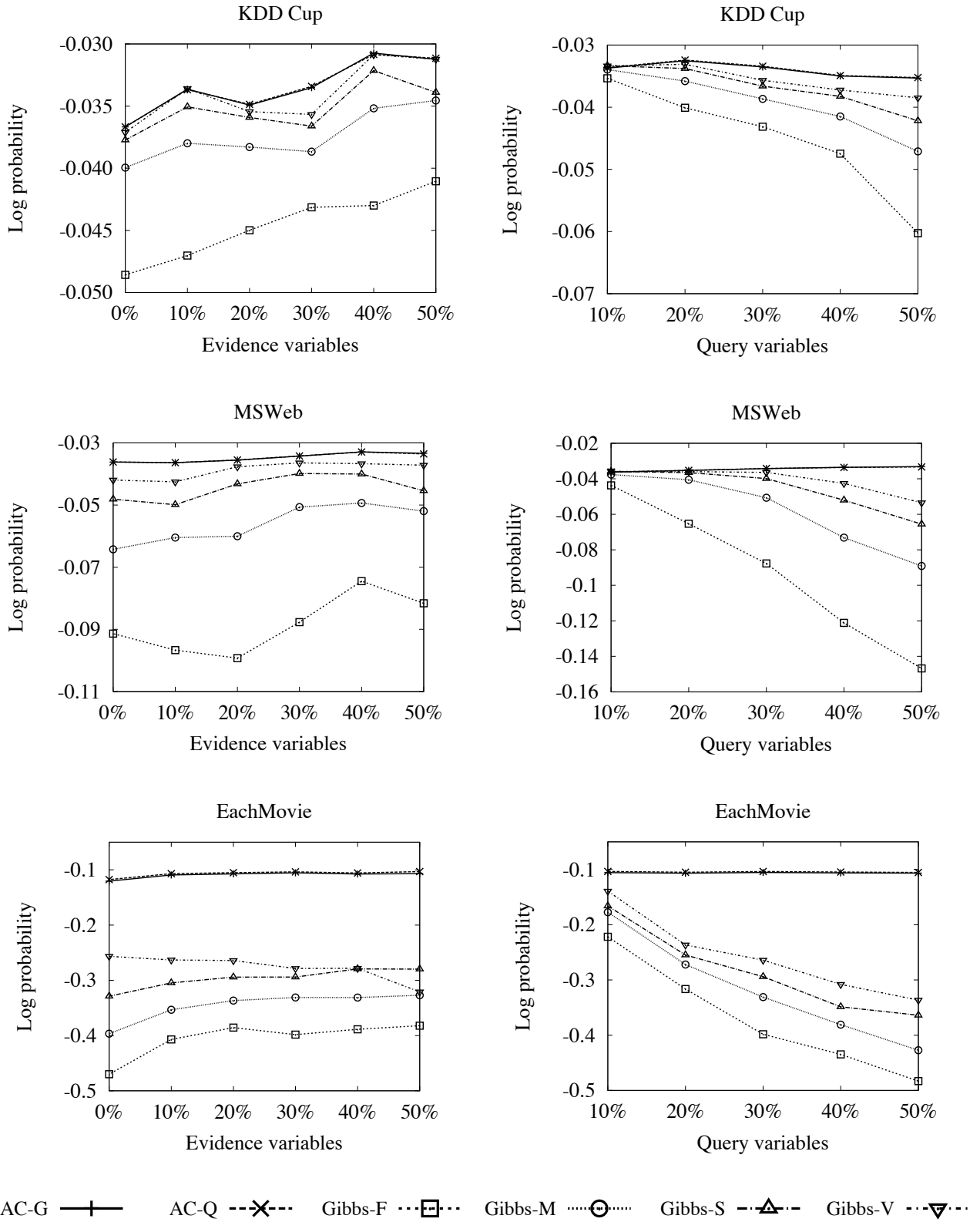
Figure 1: Conditional log probability per query variable, per query. In the legend, AC-G refers to AC-Greedy and AC-Q refers to AC-Quick. Gibbs-F, Gibbs-M, Gibbs-S and Gibbs-V refer to the fast, medium, slow, and very slow Gibbs sampling scenarios, respectively.
